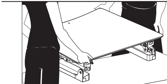
Main unit
